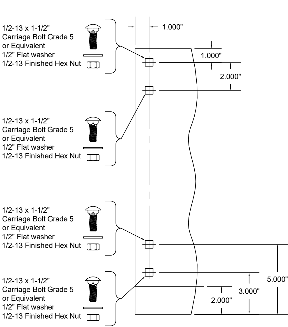
12"Ø AND LARGER SHAFT ASSEMBLY 17" AND LARGER COIL DIMENSION MIN. THICKNESS 0.240" ASTM A36 STEEL OR ASTM A480 STAINLESS STEEL, TYPES 304 OR 316, MIN. 36 KSI YIELD STRENGTH SCALE: 1-1/2" = 1'-0"
